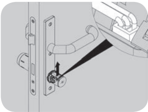
Fig. 49: Removing the battery pack
