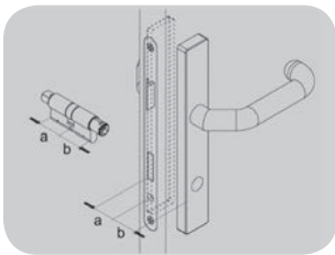
Fig. 8: Measure the thickness
