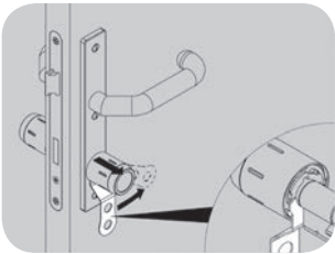
Fig. 48: Removing the knob sleeve
