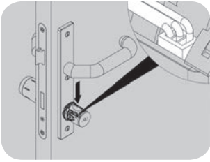
Fig. 50: Inserting the battery pack
